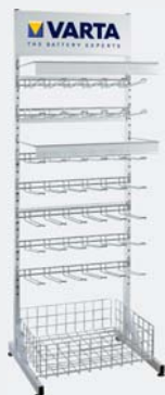
Shelf height 160 cm 1 x 9000 120 036 +1 x 9000 122 006
